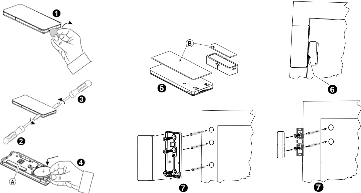
Figure 2: Mounting
